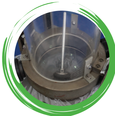
DART IMPACT TEST
